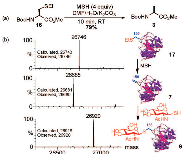
Scheme 2. MSH-Induced Oxidative Elimination Of Cys Thioethers: A Functional Switch on Protein Surfaces
