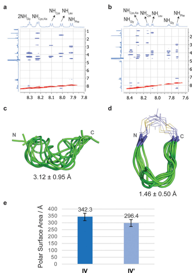
Figure 1. Conformation analysis of stapled and unstapled peptides in solution. Sections of the 500 ms ROESY spectra (400 MHz) of peptides A) IV and B) IV' in H_2O/D_2O (9:1) at pH 6.5 and 20 °C, showing amide–aliphatic crosspeaks. Structural ensembles obtained for C) peptide IV and D) stapled peptide IV' through 20-ns MD-tar simulations. The backbone is shown in green, and the carbon atoms of isobutylene moiety are in purple. The numbers indicate the rmsd for heavy-atom superimposition of the backbone with respect to the average structure. E) PSA estimated for peptides IV and IV' through the MD-tar simulations.
